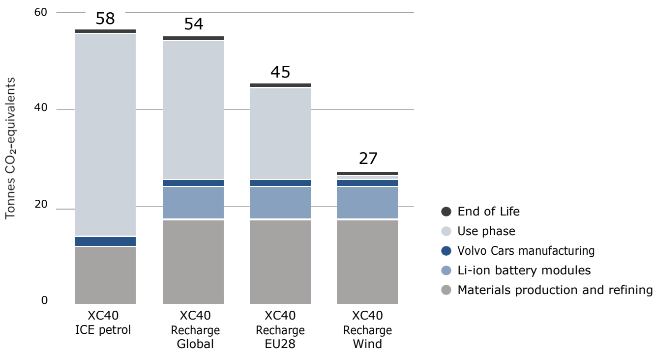
Figure i. Carbon Footprint for XC40 ICE and XC40 Recharge, with different electricity-mixes in the use phase used for the XC40 Recharge. Results are shown in tonne CO 2 -equivalents per functional unit (200 000 km lifetime range).
