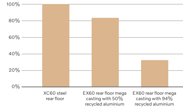
Figure 18 Carbon footprint comparison between the mega casting of the aluminium rear floor of the EX60 and the equivalent steel floor of the XC60.
