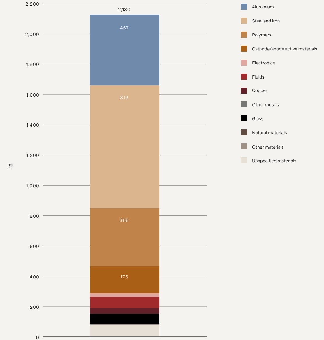
Figure 4 Material composition.
