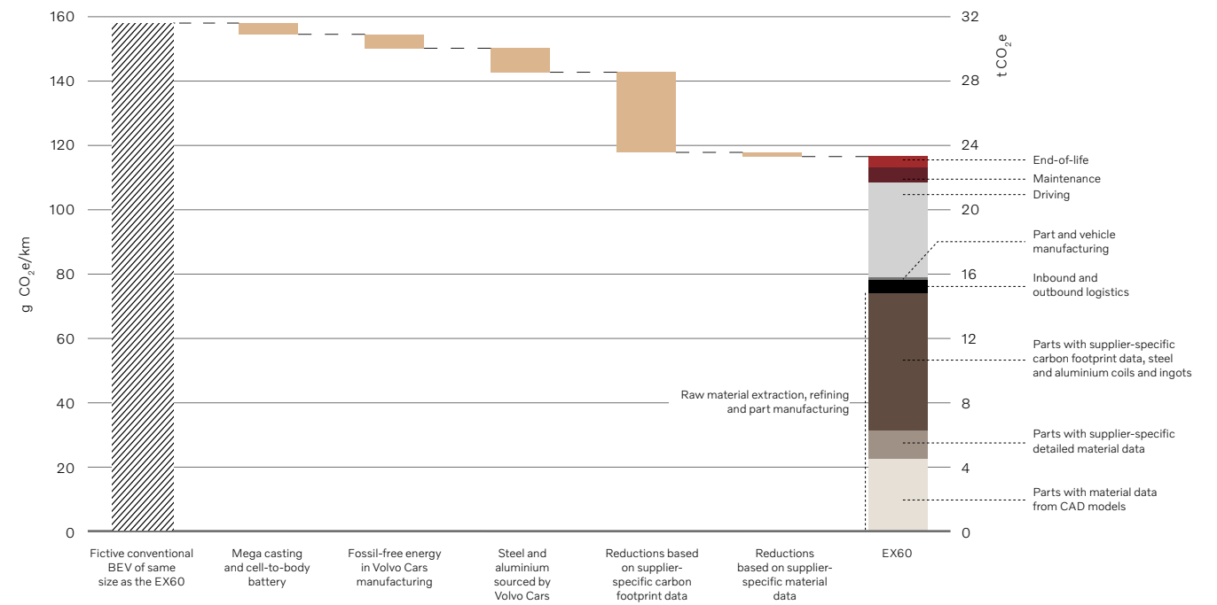
Figure i. The influence of value chain emissions reduction initiatives, specific data collection, and technological innovations on the EX60 carbon footprint when charging with European electricity mix.
