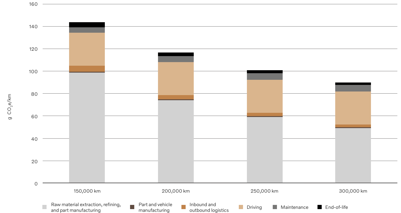
Figure 15 The effect of the lifetime distance on the carbon footprint when charging with European electricity mix.
