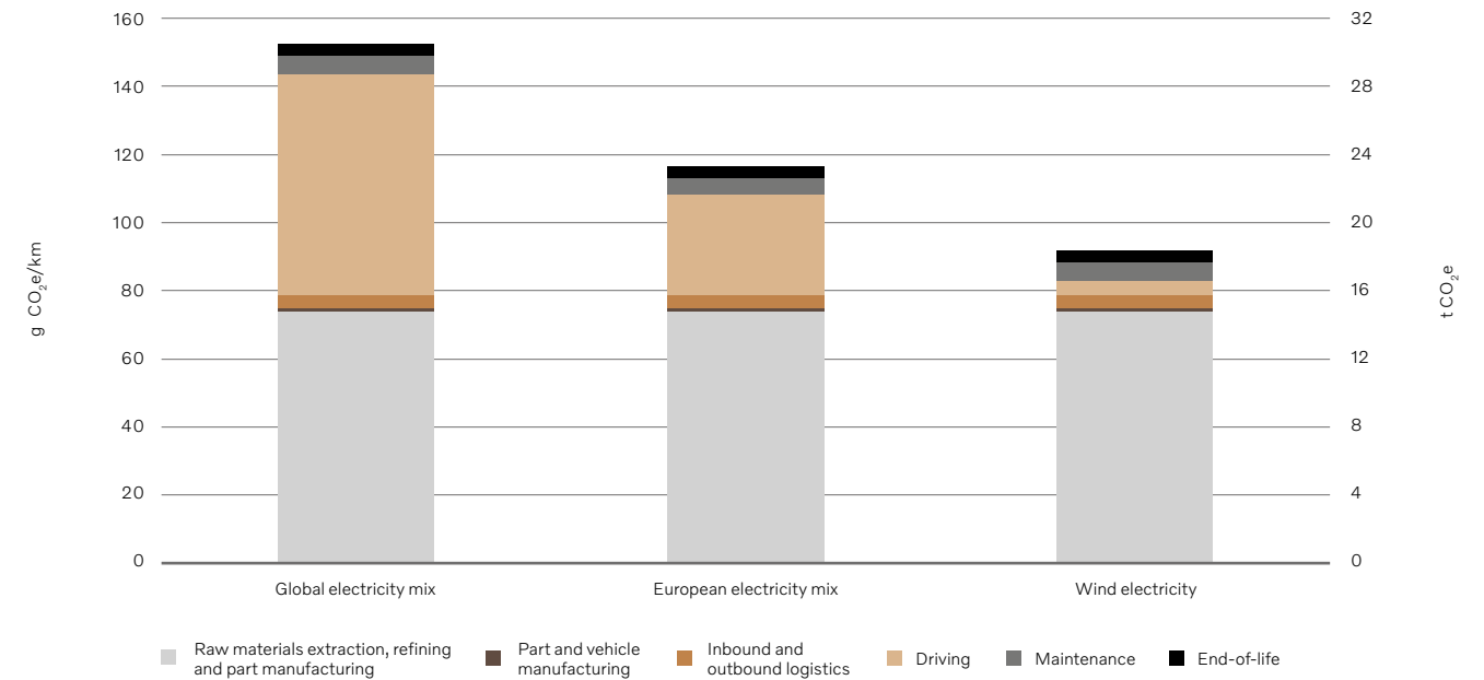
Figure 11 The EX60's carbon footprint, when charging with different electricity mixes.
