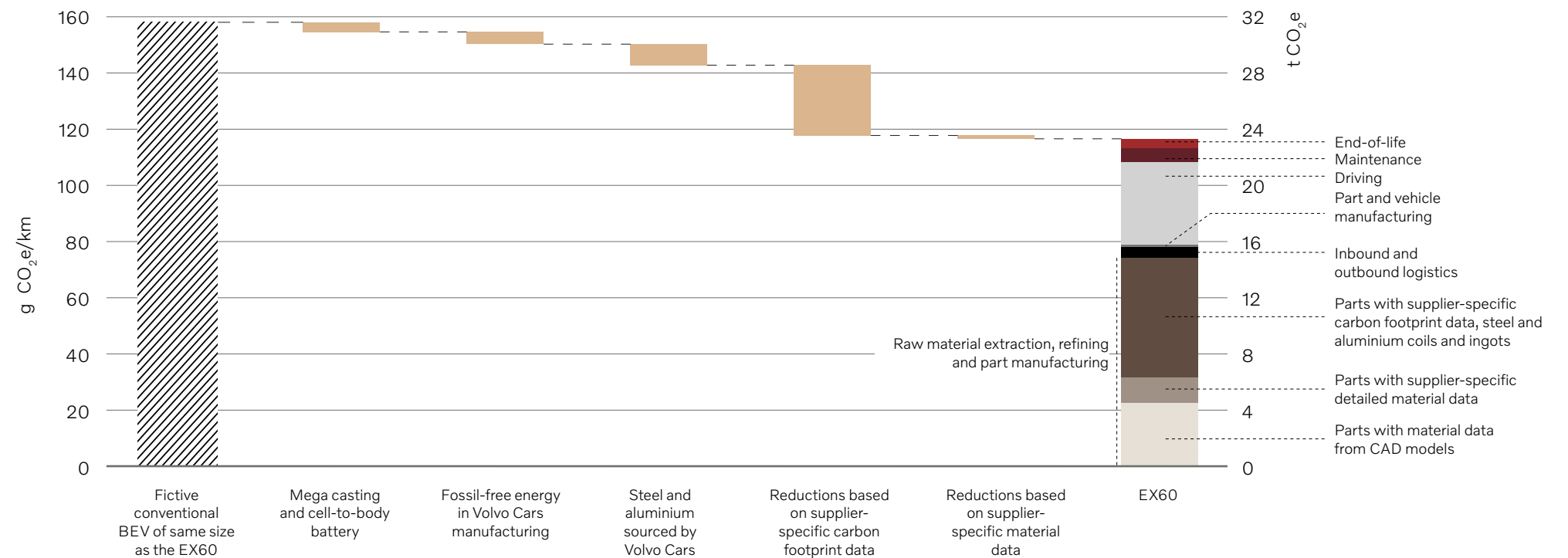
Figure 17 The influence of abatement initiatives, specific data collection, and technological innovations on the EX60 carbon footprint when charging with European electricity mix.
