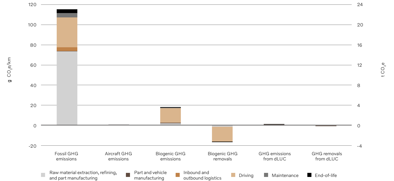
Figure 13 Specific GHG emissions and removals for the EX60 when charging with European electricity mix.
