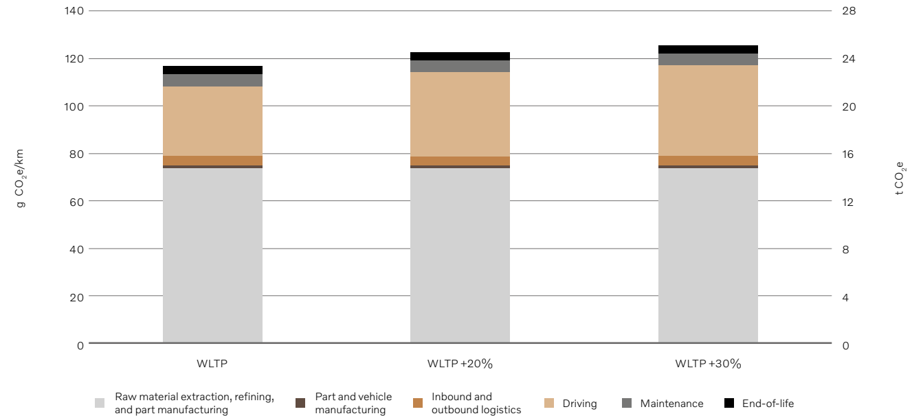
Figure 16 Carbon footprint when applying different scenarios for energy use when driving, when charging with European electricity mix.
