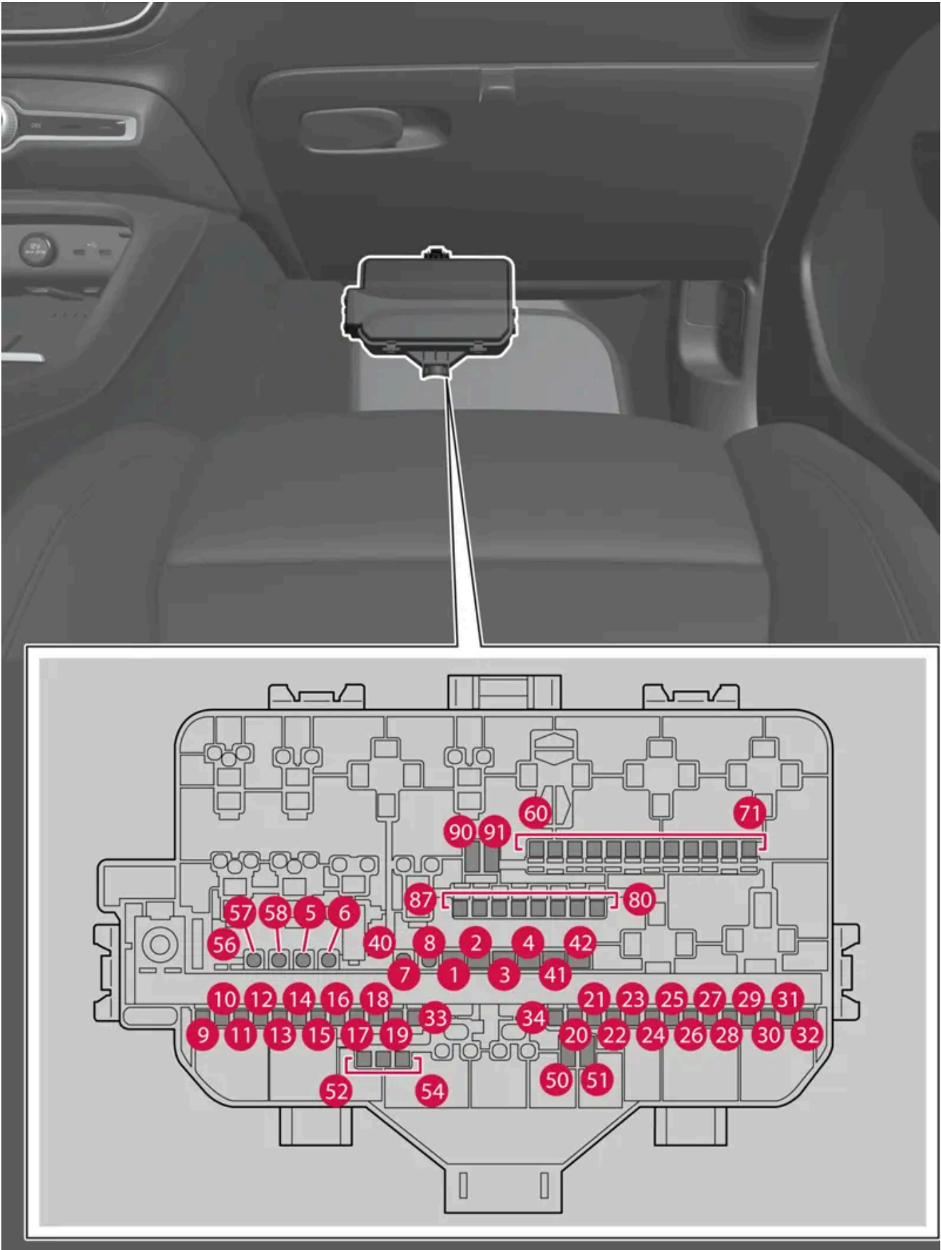
The fuse box is located behind the floor mat/panel.
