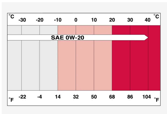
Viscosity chart
