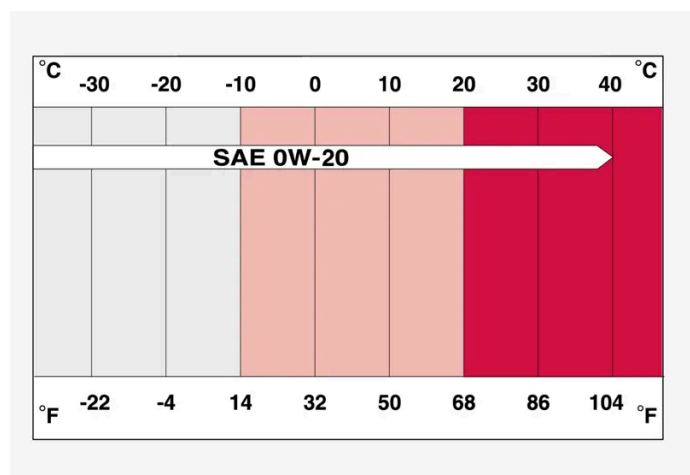
Viscosity chart
