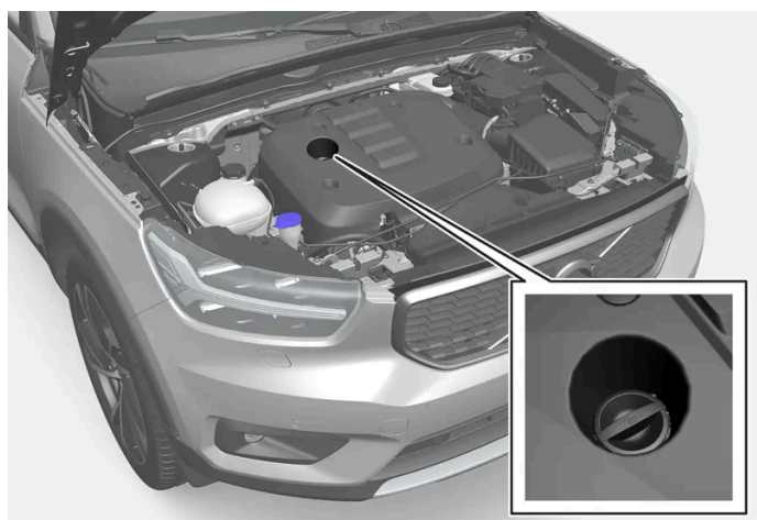
Filler pipe [1], [2]
