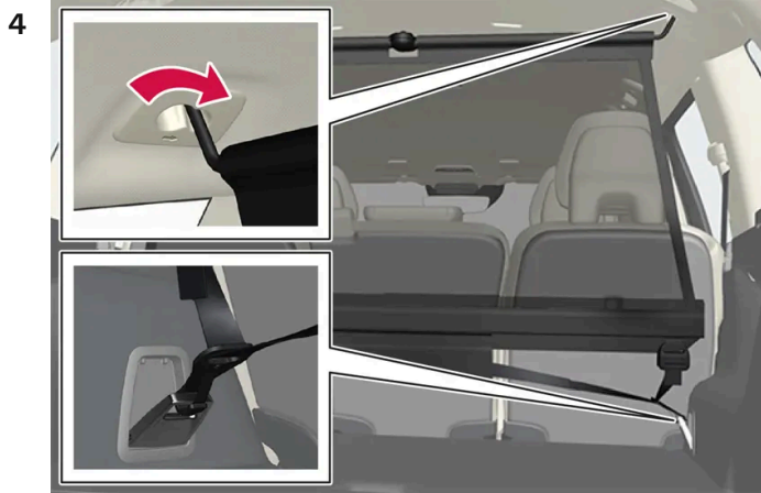
Rear mounting.
