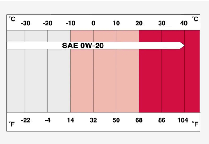
Viscosity chart
