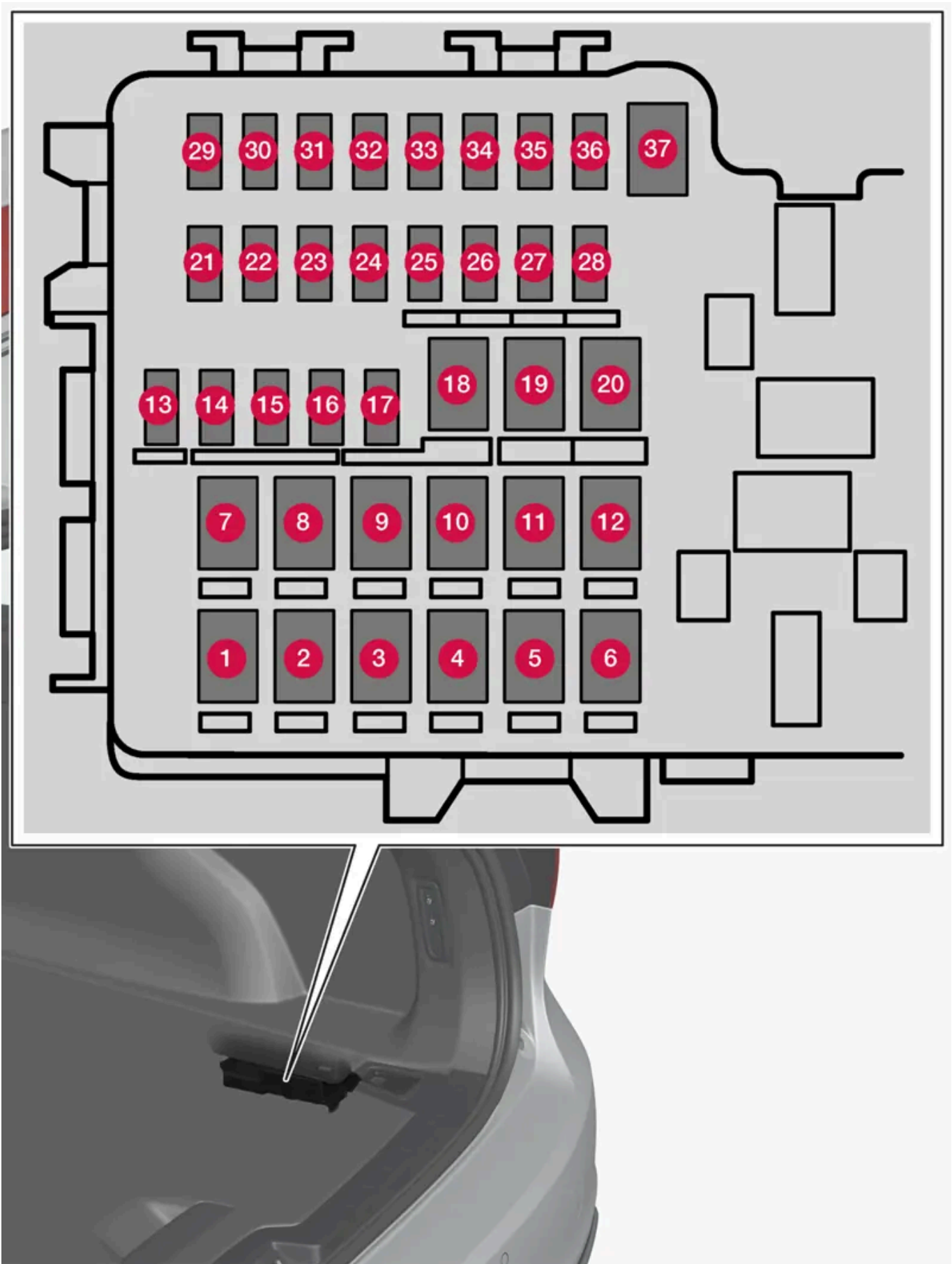
The fuse box is located behind the panel on the right-hand side.
