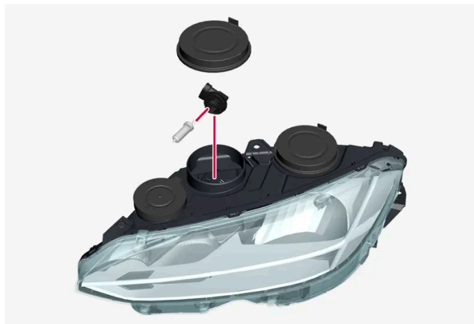
Left headlight.
