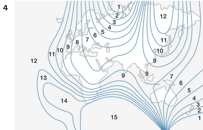
Zone magnetice.
